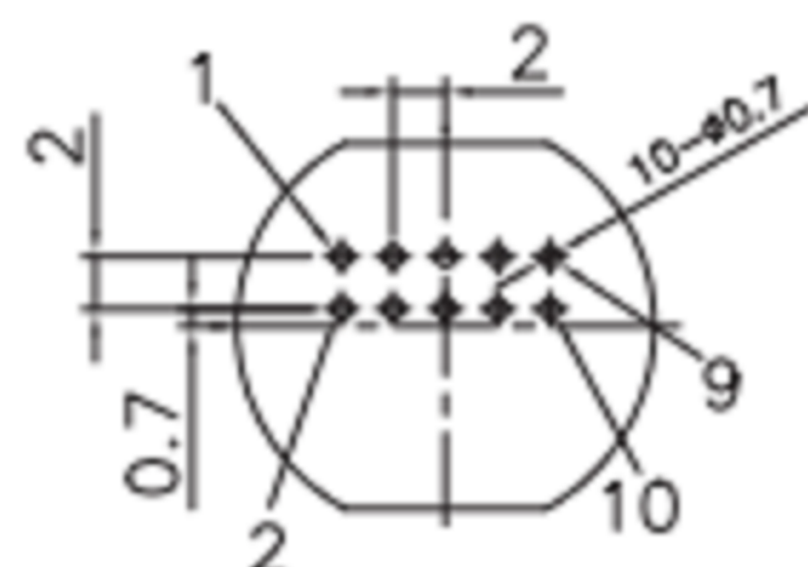
PCB开孔尺寸 PCB hole opening size
